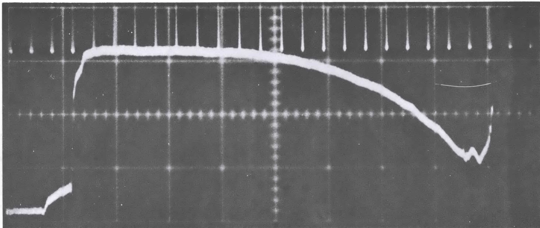
Fig. 24. Voltage-time record of a 38 kilobar final state shock wave in 6061-T6 aluminum utilizing a manganin gauge. The scale is 0.5 \mu sec/div.
